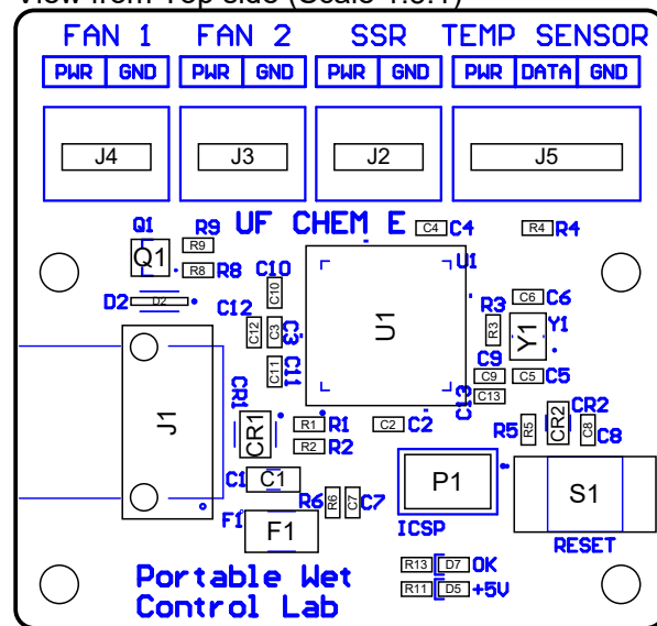
View from Top side (Scale 1.5:1)
